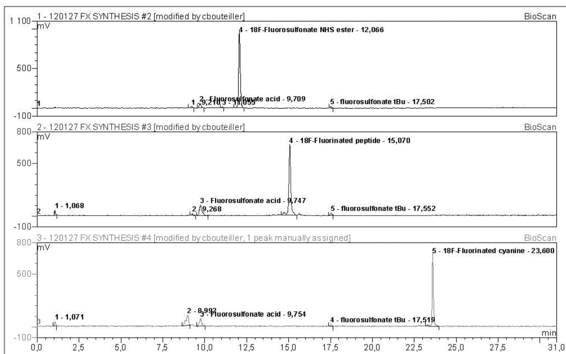
Fig. 4 Radio-HPLC elution profiles (system I) of purified [ ^{18}\text{F} ]-1 “18F-fluorosulfonate NHS ester” (top) and crude of [ ^{18}\text{F} ]-labelled dodecapeptide [ ^{18}\text{F} ]-8 “18F-fluorinated peptide” (middle) and [ ^{18}\text{F} ]-labelled cyanine [ ^{18}\text{F} ]-7 “18F-fluorinated cyanine” (bottom).
