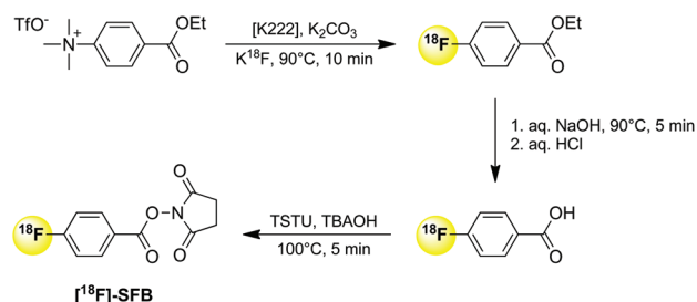
Fig. 1 General synthetic route currently used to prepare the amine-reactive [ 18 F]-labelling agent N -succinimidyl 4-[ 18 F]-fluorobenzoate ([ 18 F]-SFB). TfO - = triflate, [K222] = Kryptofix, TSTU = O -( N -succinimidyl)-1,1,3,3-tetramethyluronium tetrafluoroborate, TBAOH = tetrabutylammonium hydroxide.
